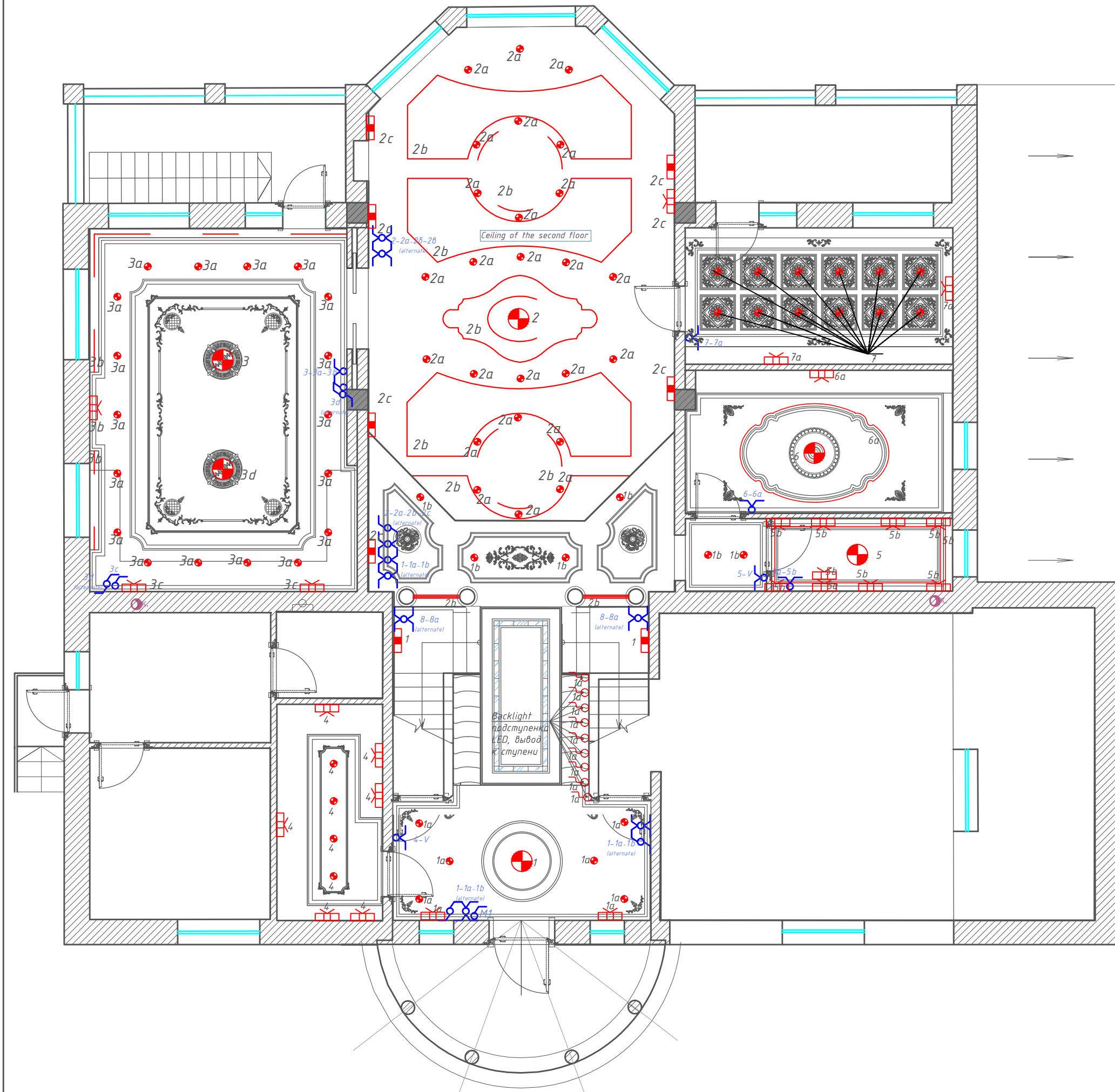
DP -17 Switches scheme 1st floor
