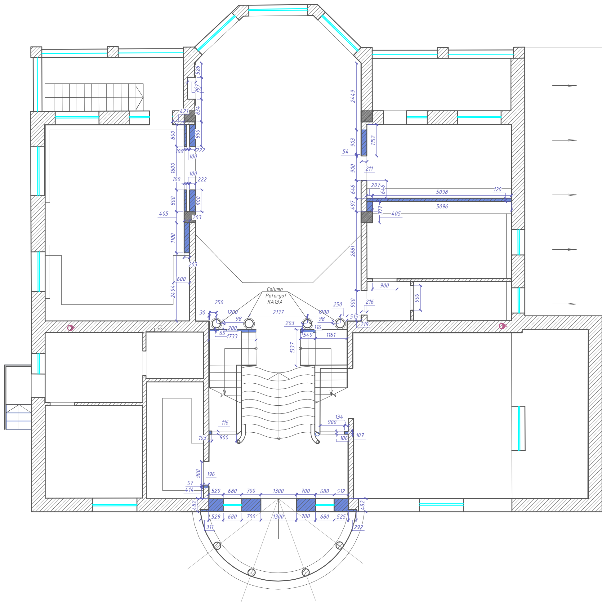
DP -3 Mounting scheme 1st floor
